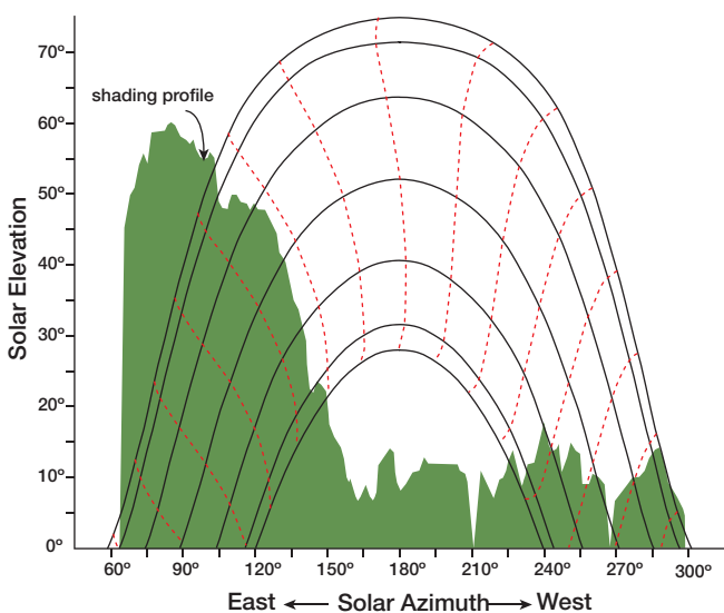
Graph 3 This graph represents a morning shade profile with sun paths superimposed.
