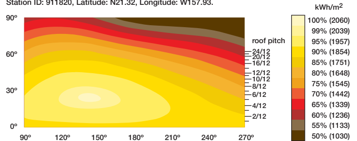
Graph 5 Annual insolation versus tilt and azimuth for Honolulu, HI, shows a significant eastward shift in the optimum annual values due to cloudy afternoon weather patterns.
