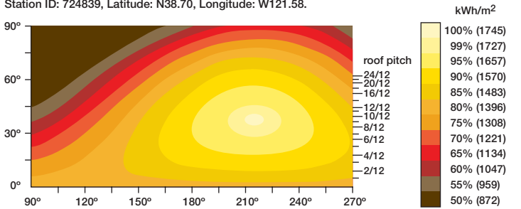
Graphs 4a & 4b Graph 4a plots the annual insolation versus tilt and azimuth for Sacramento, CA, with no shading. Graph 4b adds significant morning (eastern) shade and shows the resulting impact on insolation availability.
