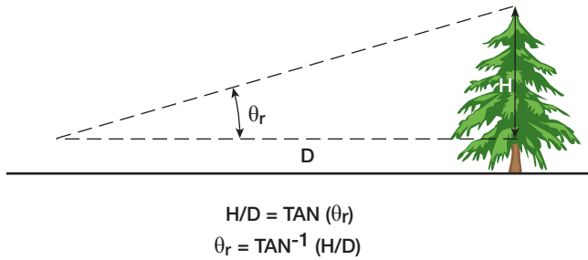
Illustration 1 To quantify shading, determine the elevation angle ( \theta ) as a function of the distance to the obstruction ( D ) and its height above the measurement plane ( H ).
